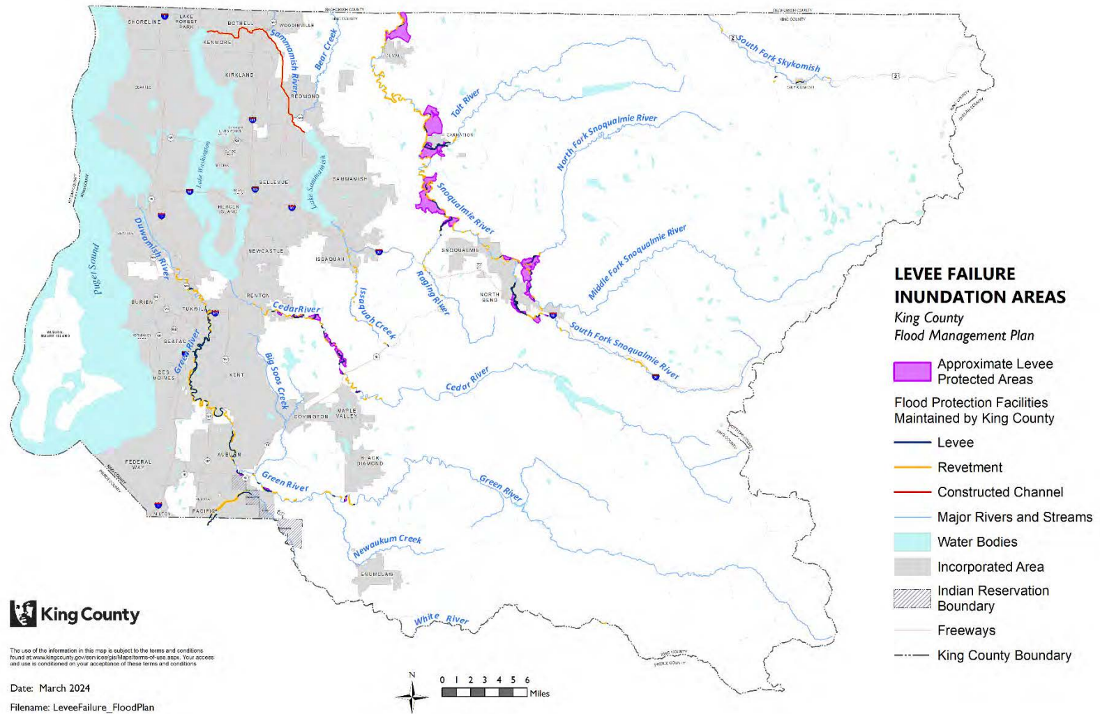
Figure D-2 Levee Failure Inundation Areas in King County
